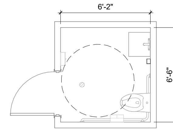
3 FIRST FLOOR ADA RESTROOM 1/4" = 1'-0"
