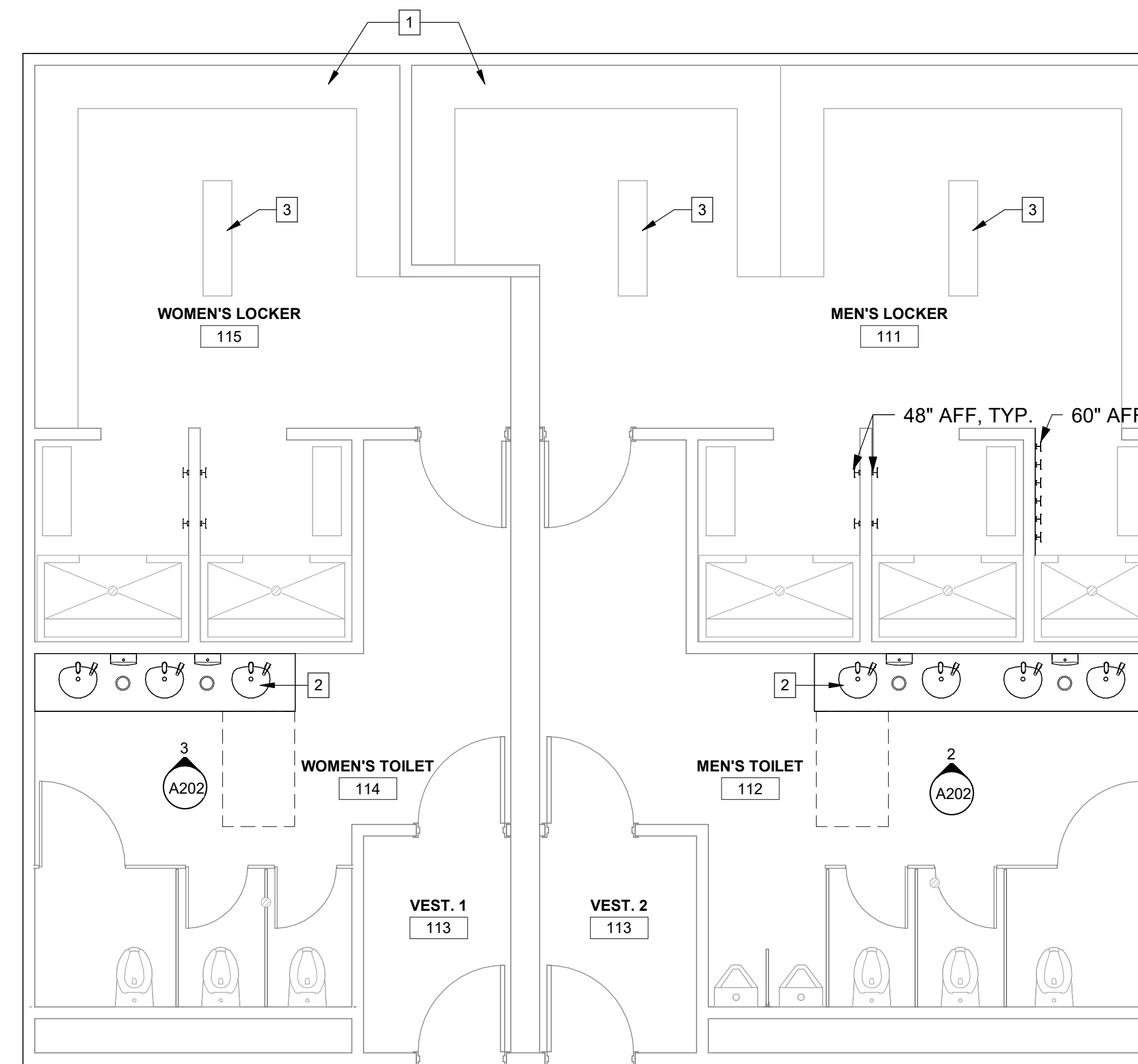
2 FIRST FLOOR OVERALL PLAN 1/4" = 1'-0"
