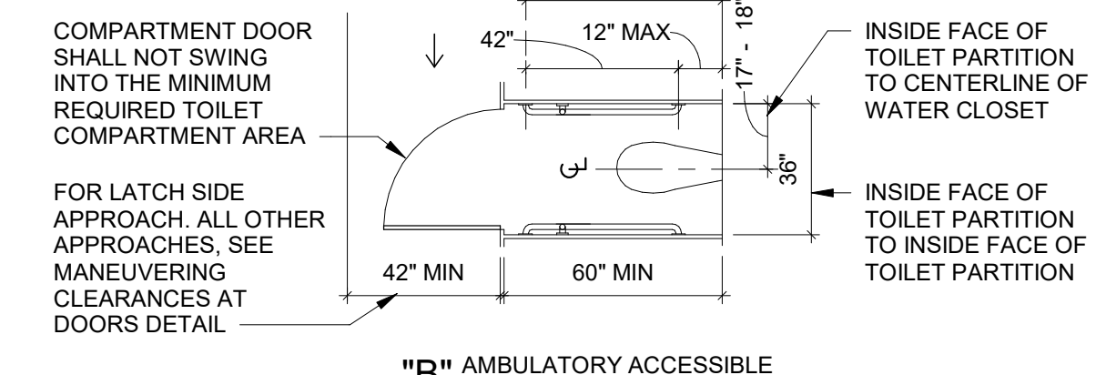
"B" AMBULATORY ACCESSIBLE STALL
