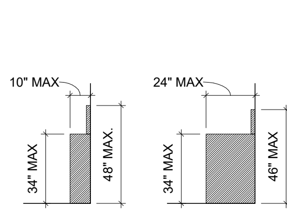
"B" OBSTRUCTED HIGH FORWARD REACH
