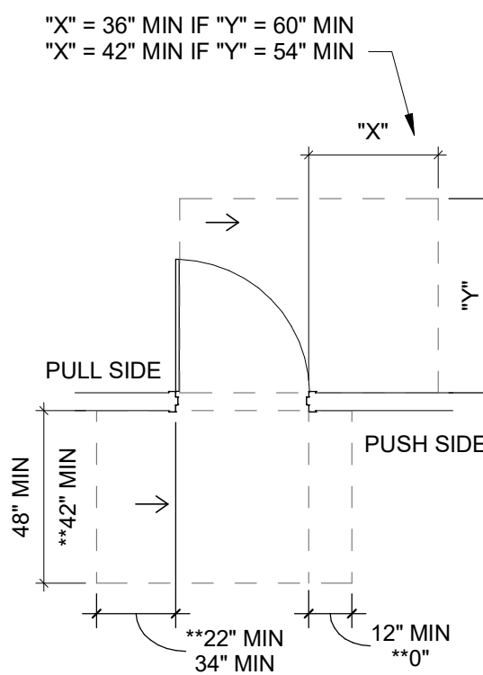
"B" MINIMUM CLEAR FLOOR SPACE FOR MANEUVERING CLEARANCE AT HINGE SIDE APPROACHES AT SWINGING DOORS
