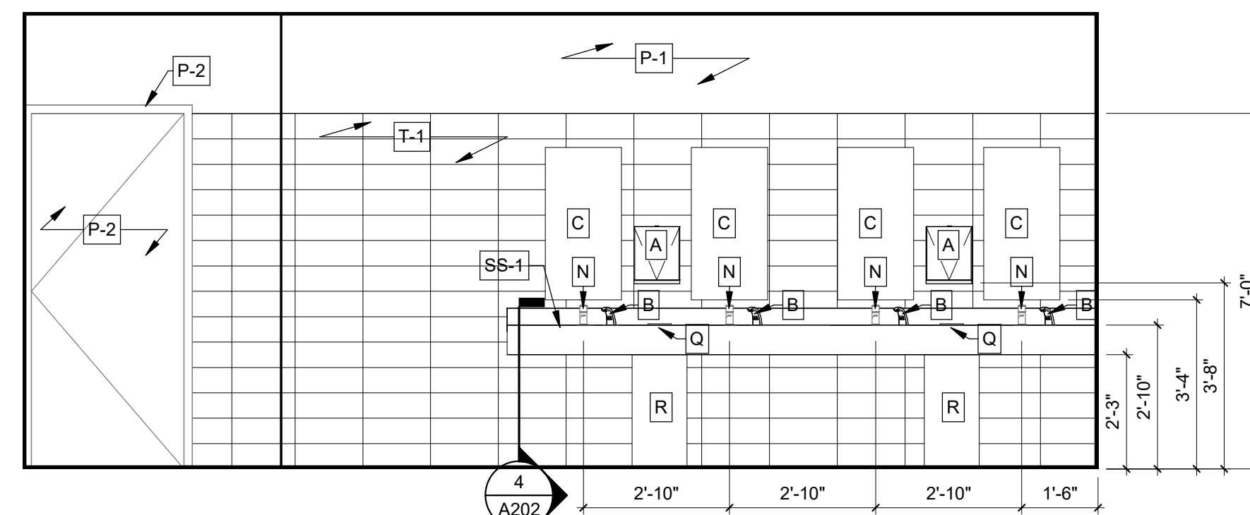
2 ELEVATION - MEN'S VANITY 3/8" = 1'-0"
