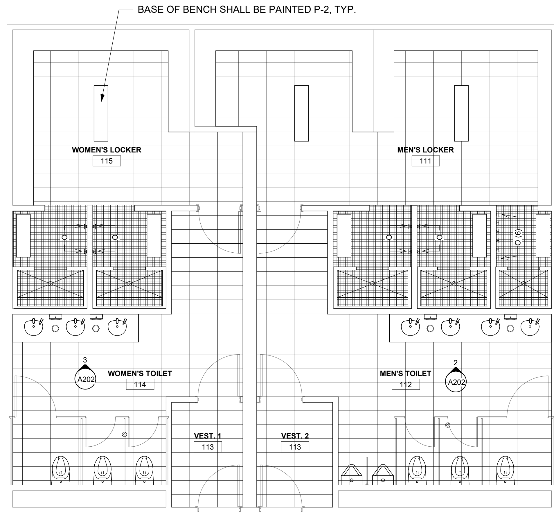
1 FIRST FLOOR FINISH PLAN 1/4" = 1'-0"
