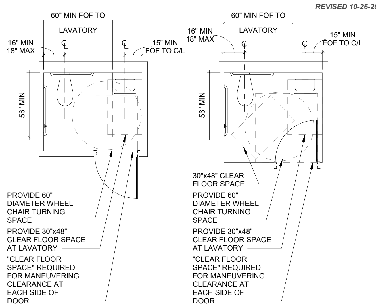
"A" TOILET ROOM WITH OUT-SWINGING DOOR "B" TOILET ROOM WITH IN-SWINGING DOOR
