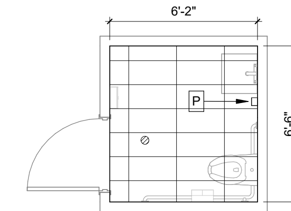
5 ADA RESTROOM FINISH PLAN 1/4" = 1'-0"
