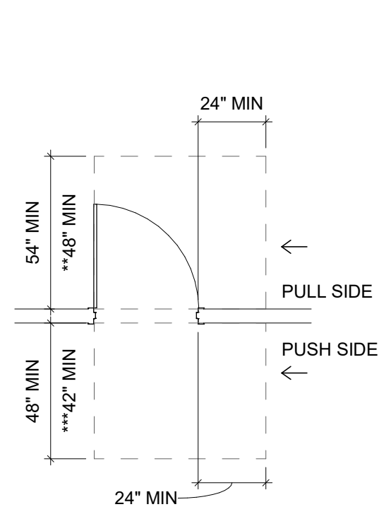
"C" MINIMUM CLEAR FLOOR SPACE FOR MANEUVERING CLEARANCE AT LATCH SIDE APPROACHES AT SWINGING DOORS
