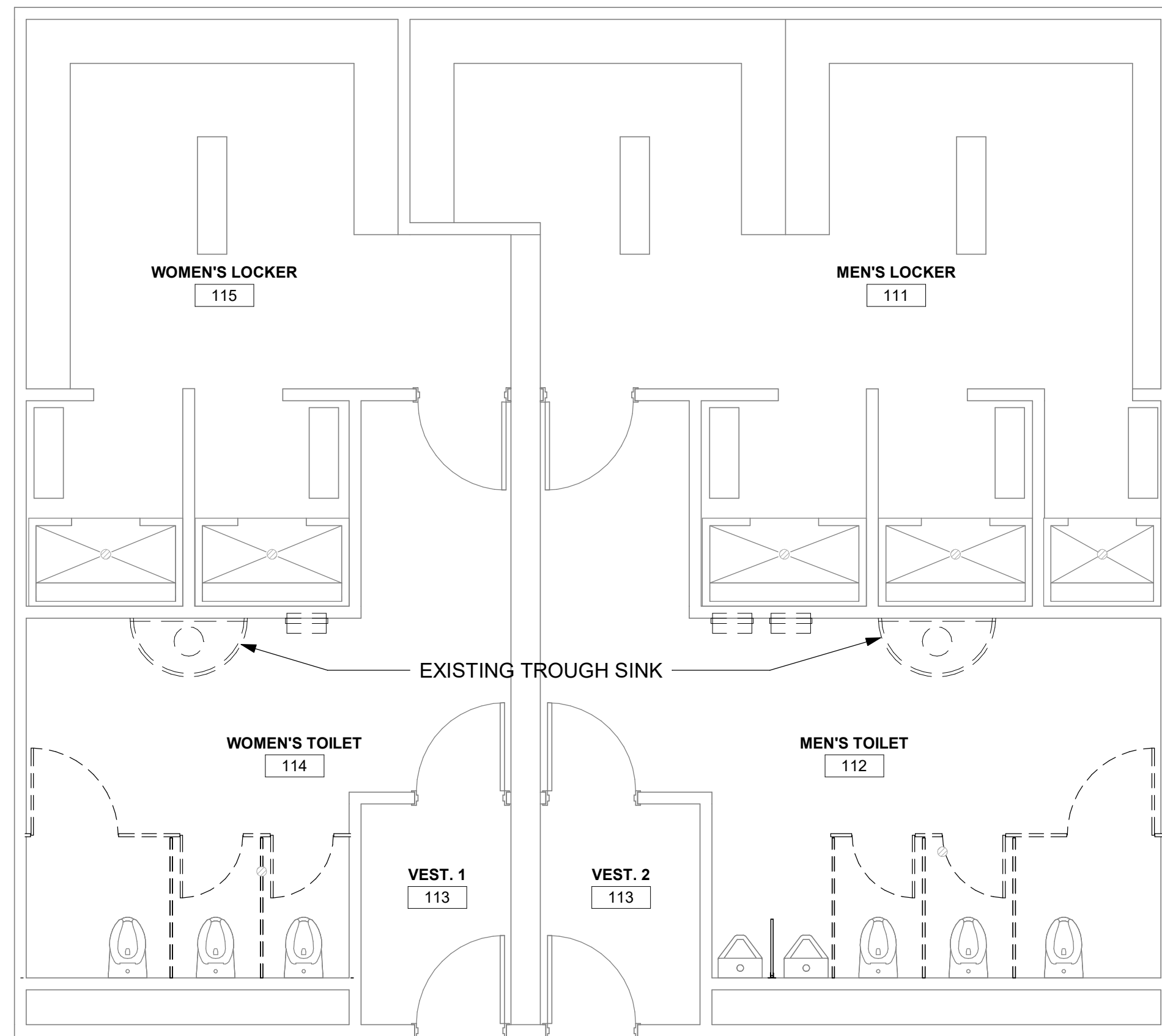
1 FIRST FLOOR DEMOLITION PLAN 1/4" = 1'-0"
