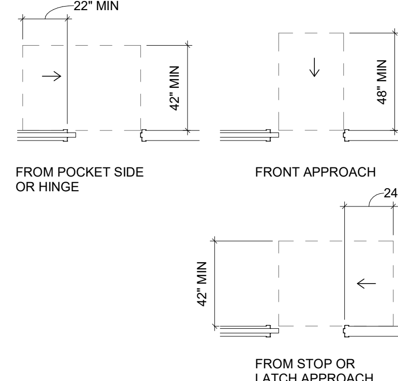
"D" MINIMUM CLEAR FLOOR SPACE FOR MANEUVERING CLEARANCE AT DOORWAYS WITHOUT DOORS, SLIDING AND FOLDING DOORS.
