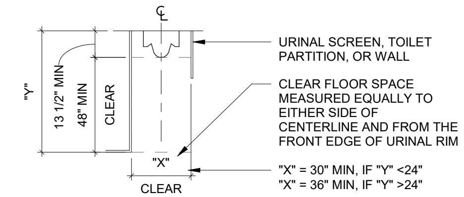
"A" URINAL FLOOR PLAN
