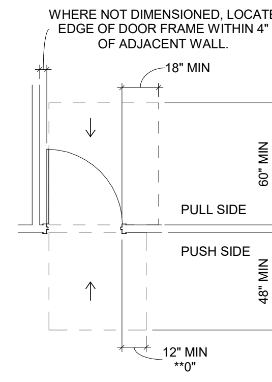
"A" MINIMUM CLEAR FLOOR SPACE FOR MANEUVERING CLEARANCE AT FRONT APPROACHES AT SWINGING DOORS
