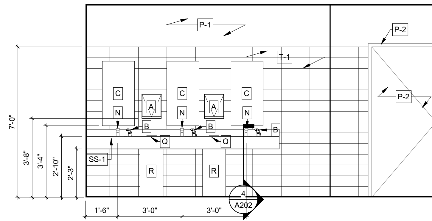
3 ELEVATION - WOMEN'S VANITY 3/8" = 1'-0"
