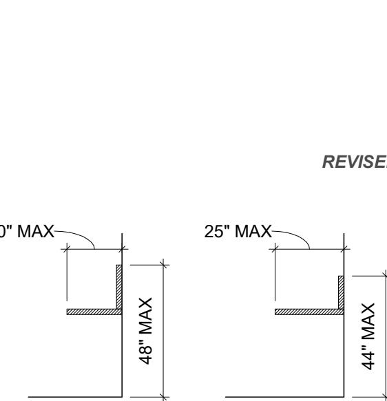
"B" OBSTRUCTED HIGH FORWARD REACH
