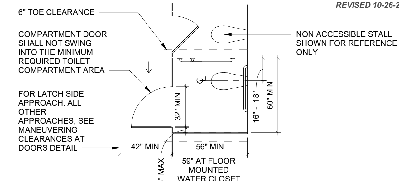
"A" WHEELCHAIR ACCESSIBLE STALL
