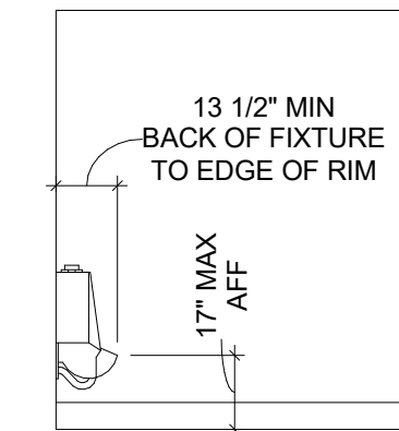
"B" URINAL ELEVATION
