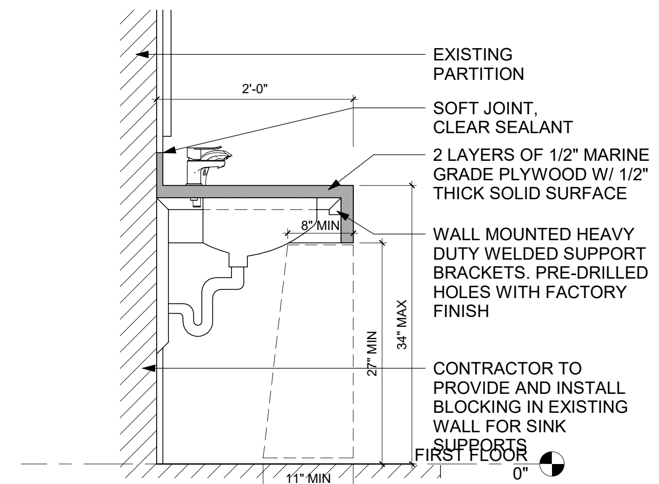
4 SECTION AT SINK 1" = 1'-0"
